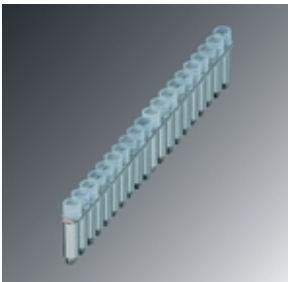
Fixed bridge, pitch: 5 mm, number of positions: 20, color: silver
